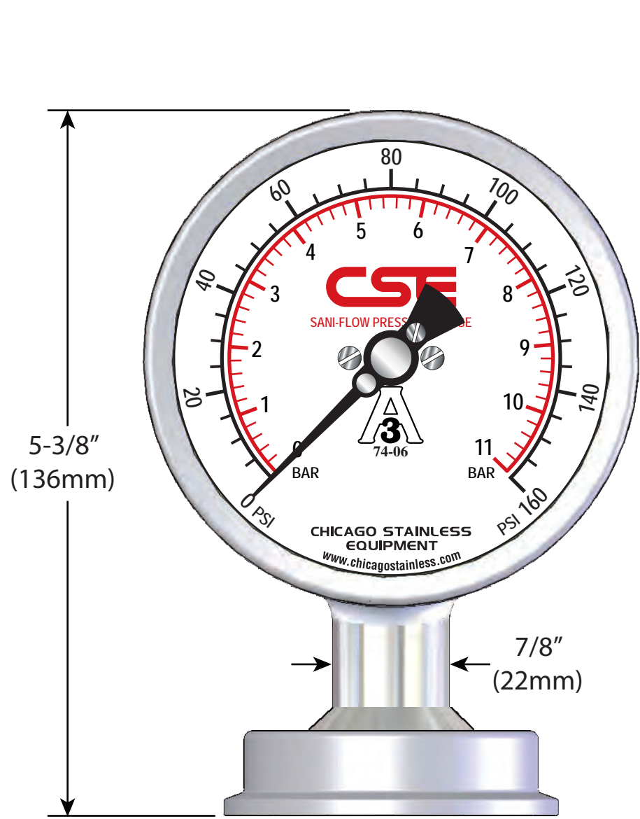
3-1/2" BOTTOM MOUNT (Shown with 2" Tri-Clamp)
