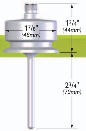
1 1/2" Tri-Clamp Transmitter
