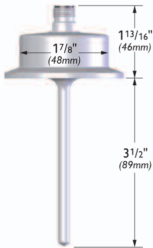
2" Tri-Clamp Transmitter
