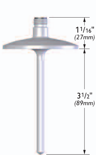
2" Tri-Clamp RTD
