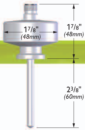
3/4" Tri-Clamp Transmitter
