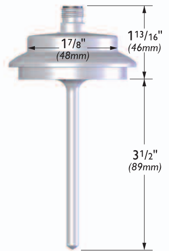
2" I-Line Transmitter
